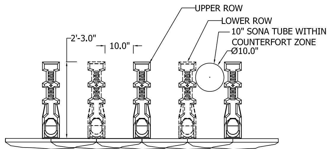
PLAN VIEW DETAIL (2 ROWS SHOWN)
