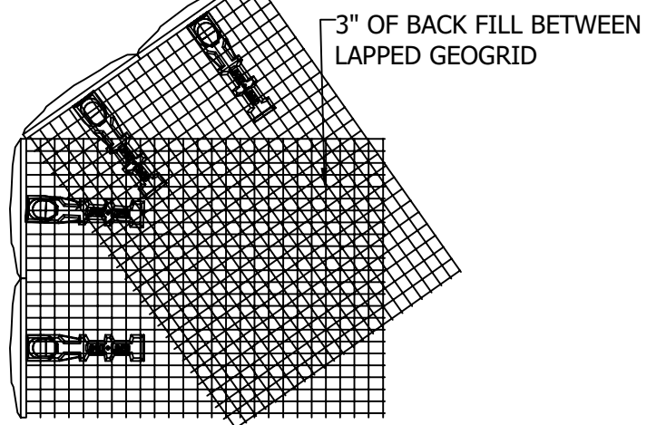
PLAN VIEW OBTUSE OUTSIDE CORNER 90-180 DEGREES
